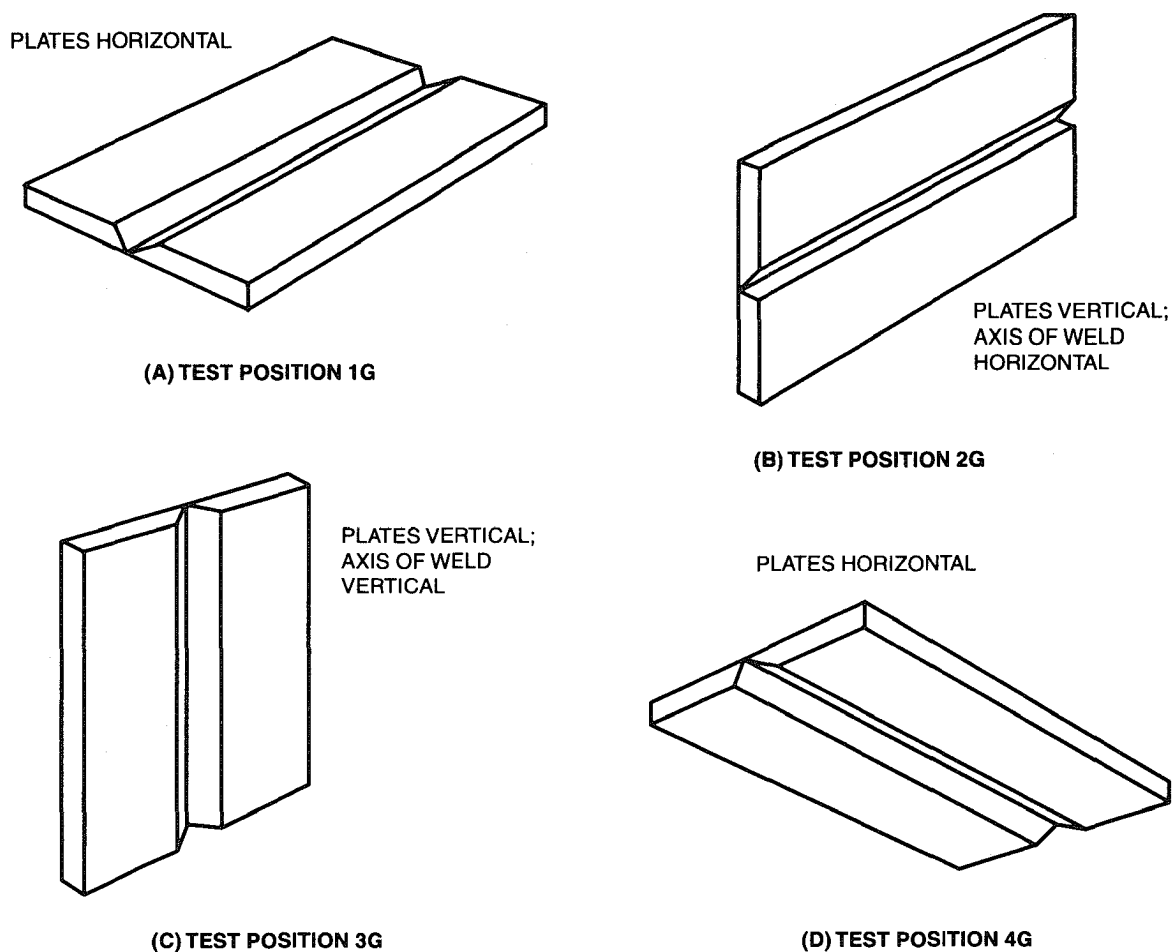
Figure 4.3—Positions of Test Plates for Groove Welds (see 4.2.4)
