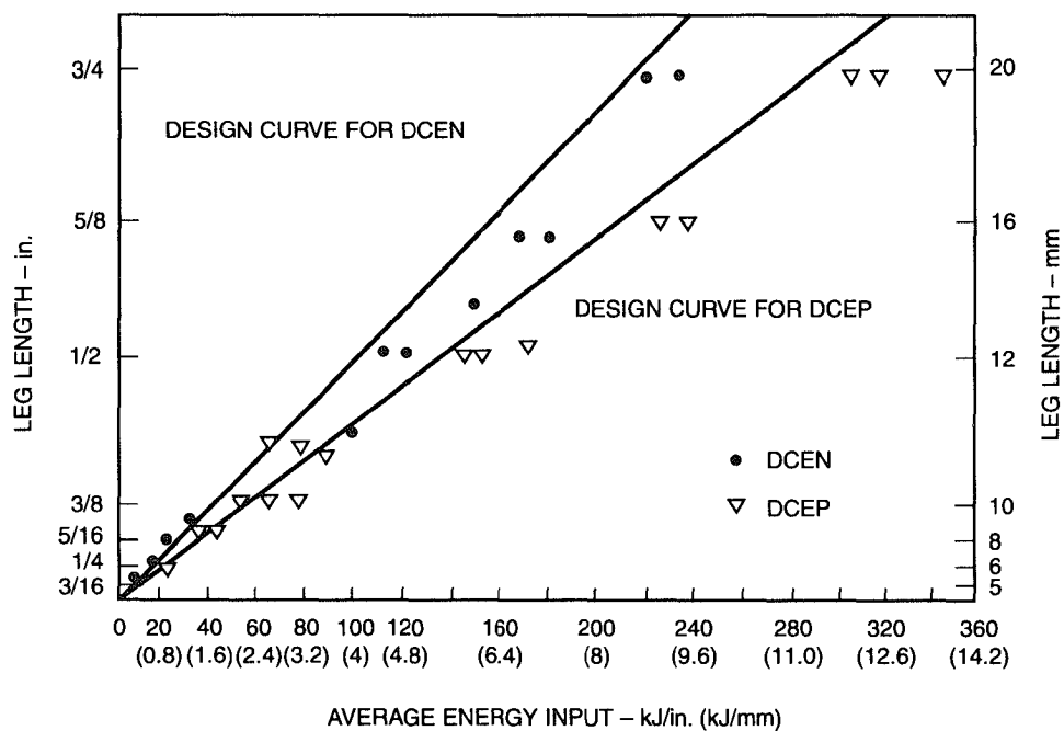
Figure XI-4—Relation Between Fillet Weld Size and Energy Input (see XI16.1.5)
