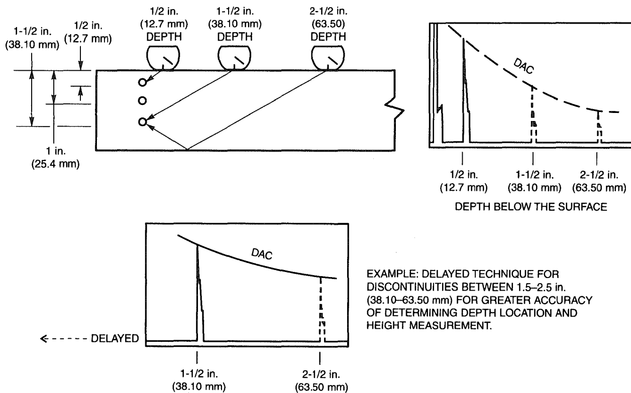
Figure K-7—Shear Wave Distance and Sensitivity Calibration (see K6.3.1)
