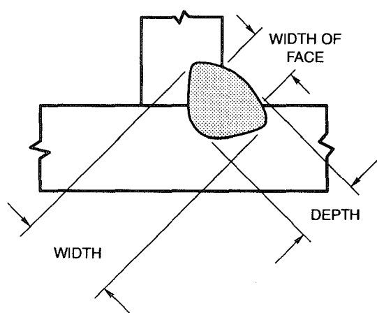
Figure 3.1—Weld Bead in which Depth and Width Exceed the Width of the Weld Face (see 3.7.2)
