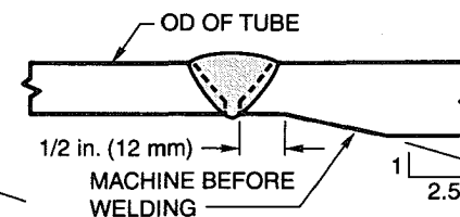
(E) TRANSITION BY STRAIGHT AND TAPER BORE AT THICKER TUBE
