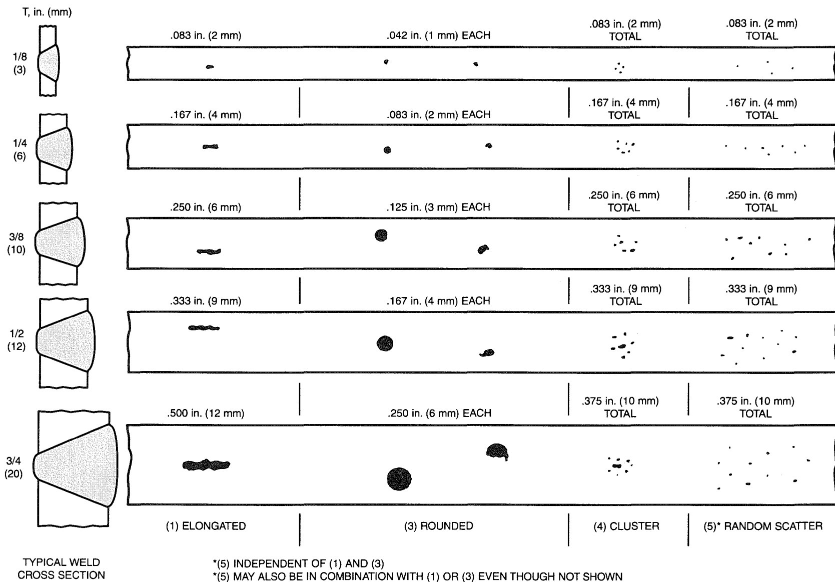
Figure 6.2—Maximum Acceptable Radiographic Images Per 6.12.3.1 (see 6.12.1.2 and 6.12.3.2)
