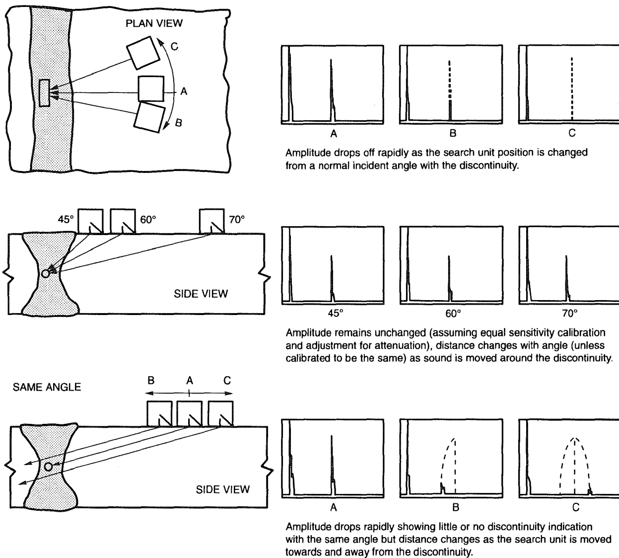
Figure K-10—Cylindrical Discontinuity Characteristics (see K8.2.2)
