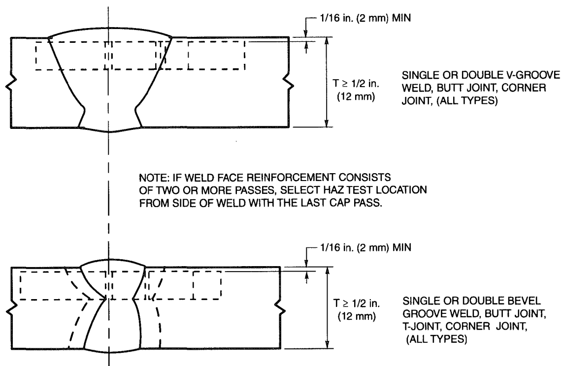
Figure III-1—Location of WPS Charpy Specimens (see III2.1)
