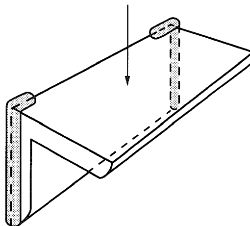
(B) BOXING AROUND TOP OF SEAT ANGLE CONNECTIONS
