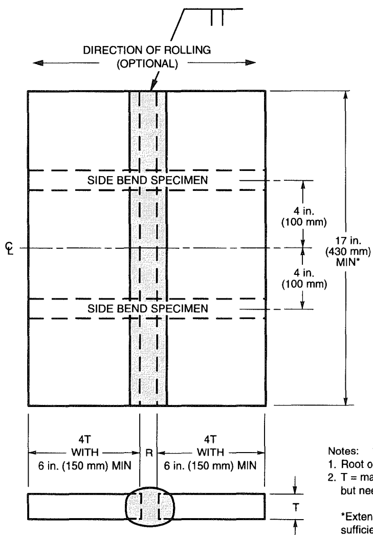
Figure 4.35—Butt Joint for Welding Operator Qualification— Electroslag and Electrode Gas Welding (see 4.23.2)
