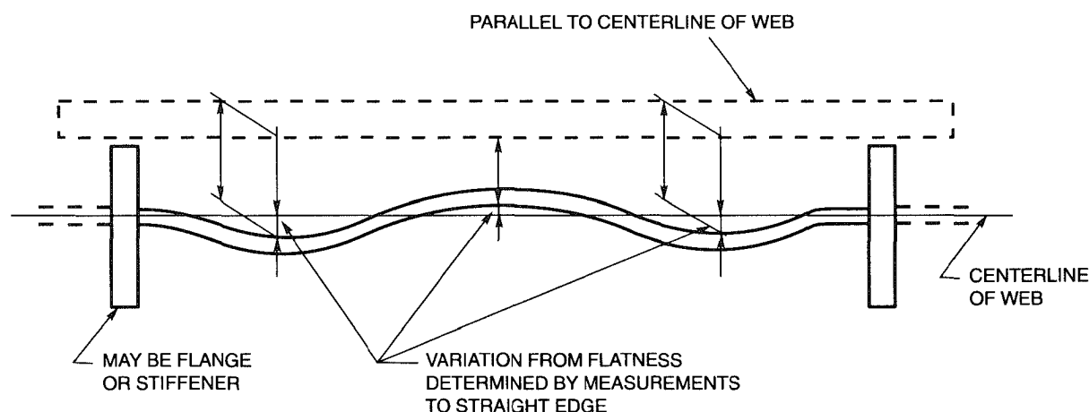
Figure C5.5—Typical Method to Determine Variations in Girder Web Flatness (see C5.23.6.1)
