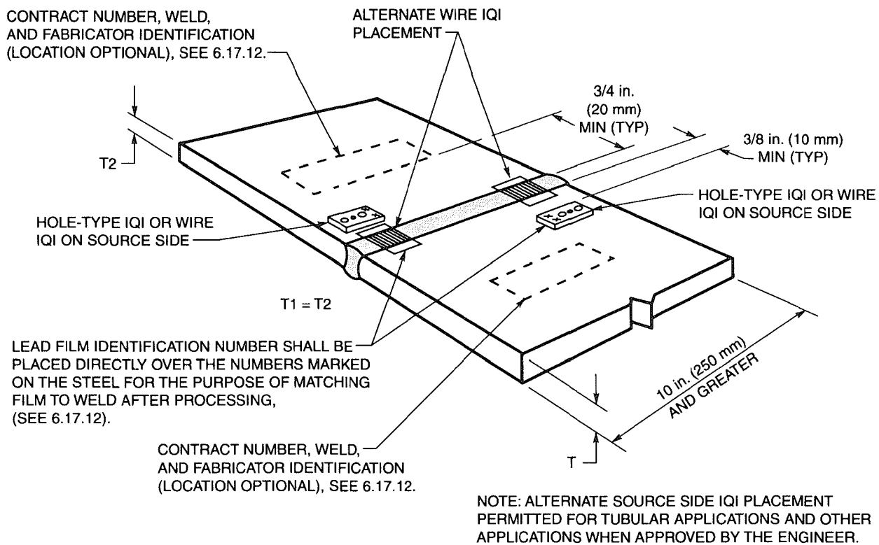
Figure 6.11—Radiographic Identification and Hole-Type or Wire IQI Locations on Approximately Equal Thickness Joints 10 in. (250 mm) and Greater in Length (see 6.17.7)
