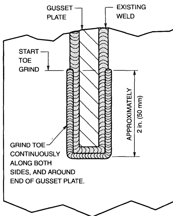
Figure C8.4—Toe Dressing Normal to Stress (see C8.4.1)
