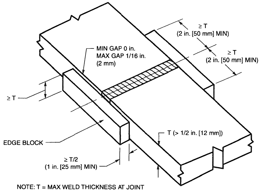
Figure 6.15—Radiographic Edge Blocks (see 6.17.13)
