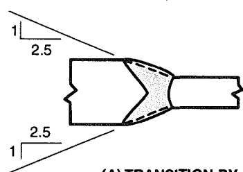
(A) TRANSITION BY SLOPING WELD SURFACE
