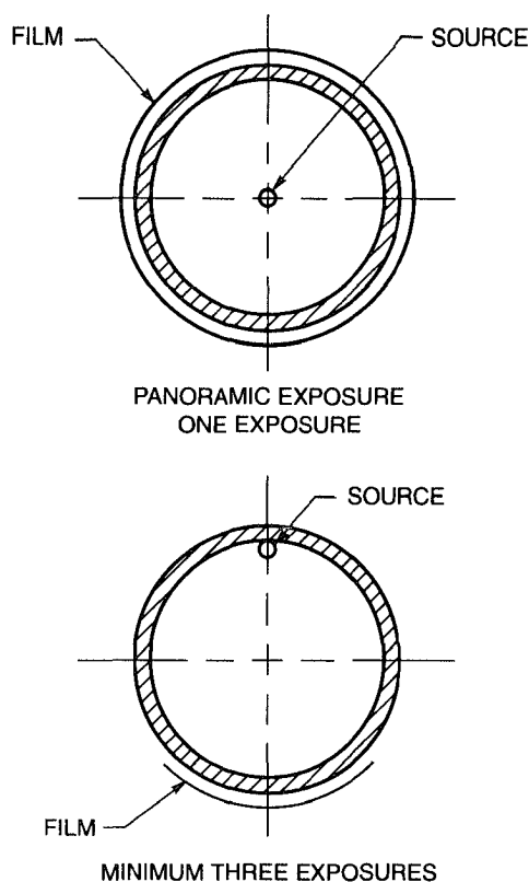
Figure 6.16—Single-Wall Exposure— Single-Wall View (see 6.18.1.1)
