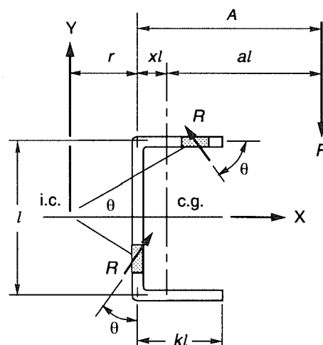
Figure C2.5—Eccentric Loading (see C2.14.4 and C2.14.5)
