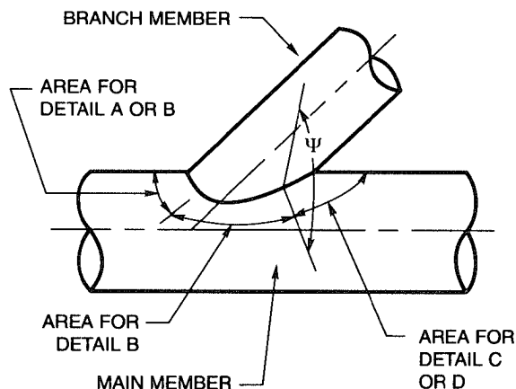
Figure 3.7—Definitions and Detailed Selections for Prequalified CJP T-, Y-, and K-Tubular Connections (see 3.13.4 and Table 3.5)
