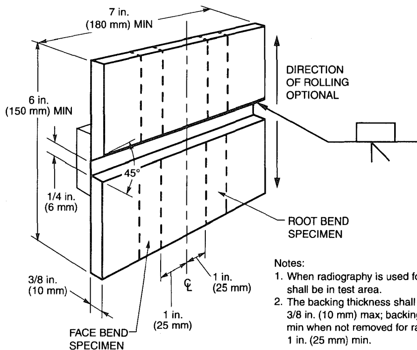
Figure 4.31—Optional Test Plate for Limited Thickness—Horizontal Position—Welder Qualification (see 4.23.1)
