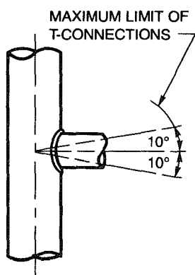
(C) T-CONNECTION
