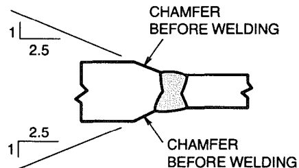
(C) TRANSITION BY CHAMFERING THICKER PART
