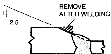
(A) TRANSITION BY SLOPING WELD SURFACE
