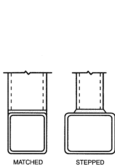
(L) CONNECTION TYPES FOR BOX SECTIONS
