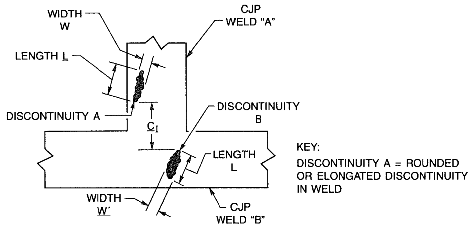
CASE III DISCONTINUITY LIMITATIONS
