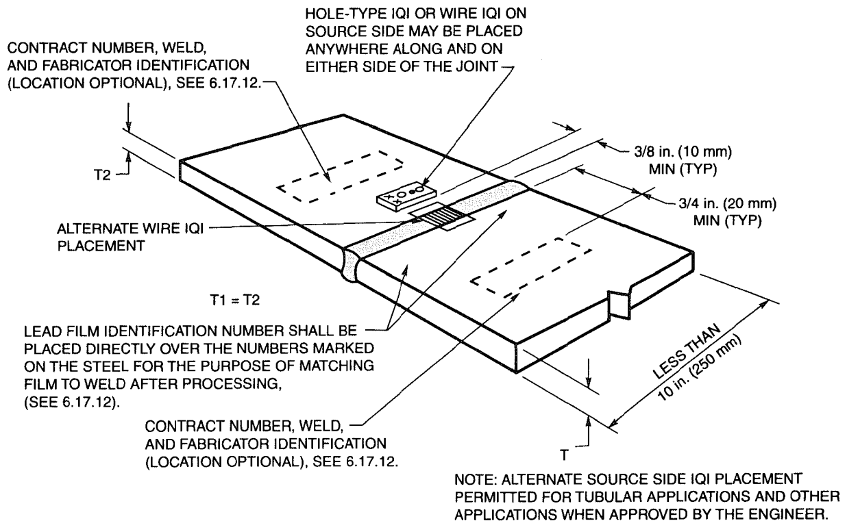
Figure 6.12—Radiographic Identification and Hole-Type or Wire IQI Locations on Approximately Equal Thickness Joints Less Than 10 in. (250 mm) in Length (see 6.17.7)
