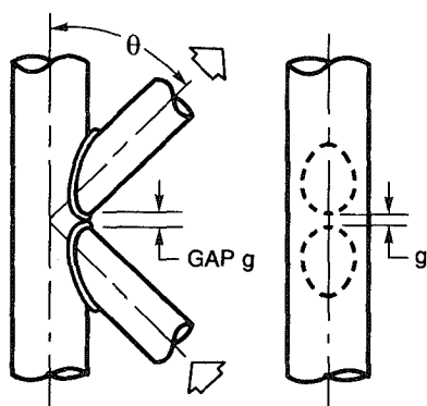
(E) K-CONNECTION
