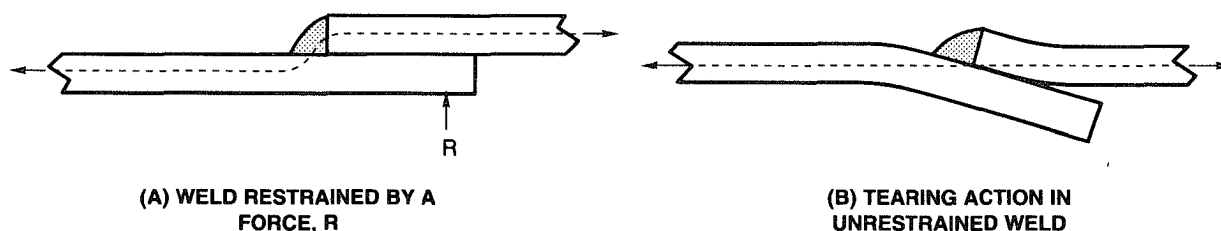
Figure C2.14—Single Fillet Welded Lap Joints (see C2.4.8.1)
