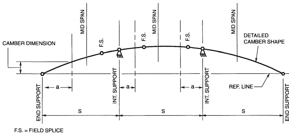
TYPICAL GIRDER ASSEMBLY
