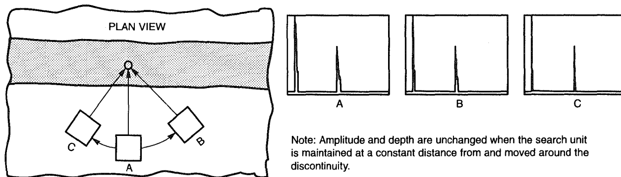
Figure K-9—Spherical Discontinuity Characteristics (see K8.2.1)
