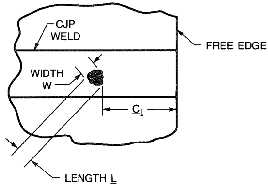
CASE II DISCONTINUITY LIMITATIONS
