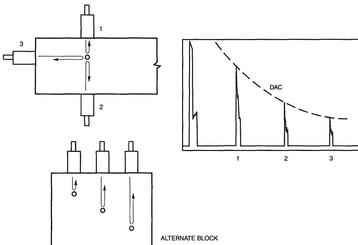
Figure K-6—Compression Wave Sensitivity Calibration (see K6.2.2)
