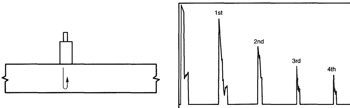
Figure K-5—Compression Wave Depth (Horizontal Sweep Calibration) (see K6.2.1)
