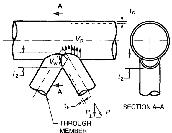
Figure 2.18—Detail of Overlapping Joint (see 2.40.1.6)
