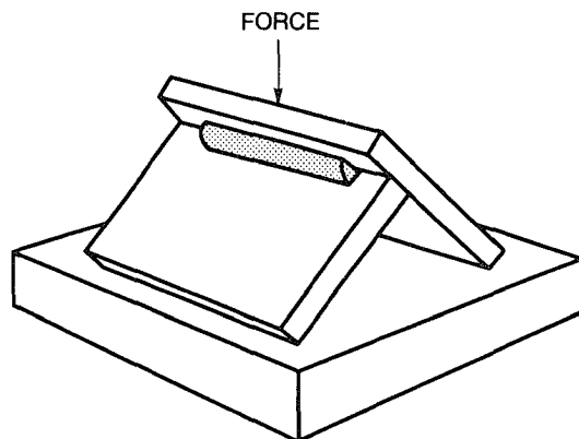
Figure 4.34—Method of Rupturing Specimen— Tack Welder Qualification (see 4.31)
