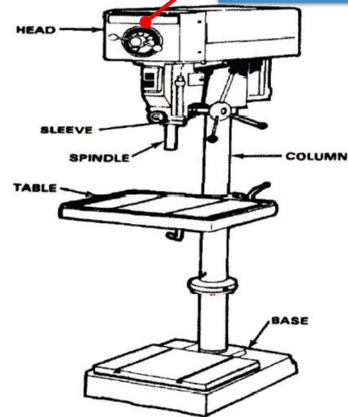
Fig. 8 Components of an upright drilling machine
